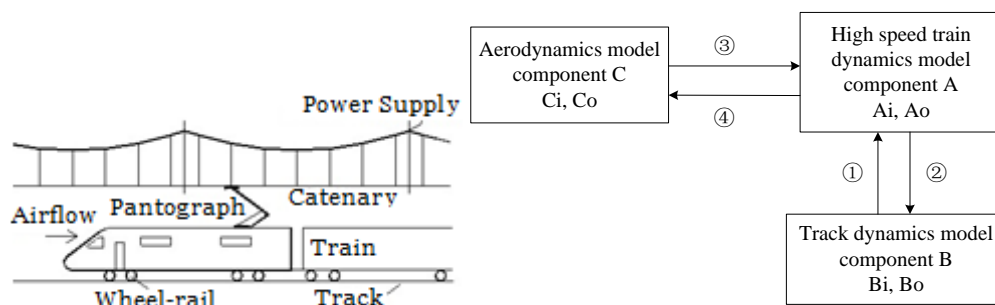
Fig.4 High speed train-track-airflow coupled modeling
