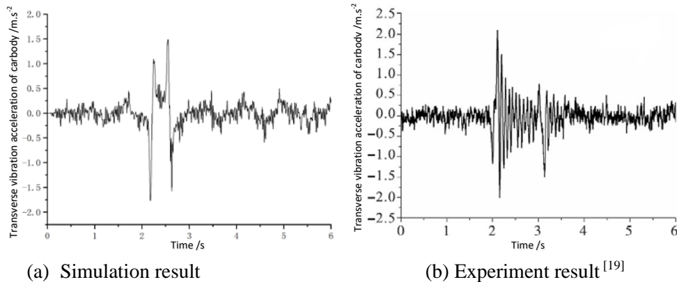
Fig.7 Transverse vibration acceleration of left-front test point on car body of head train with meeting speed of 350km/h
