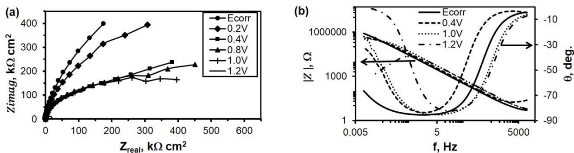
Figure 6. (a) Complex plane plots, and (b) Bode plots of amorphous Ti-51at.%Ni TiNi films in PBS solution at 37°C. For clarity, data are not shown for all potentials.
