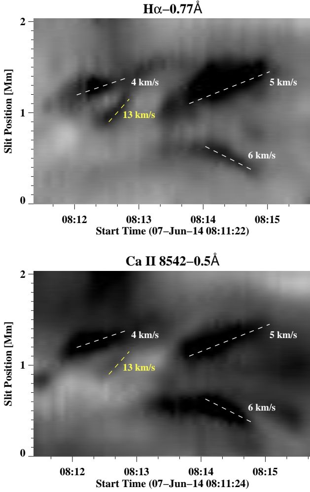
Fig. 5. Space-time slice image of (a) H\alpha-0.77 \text{ \AA} intensity and (b) \text{Ca II } 8542-0.5 \text{ \AA} intensity along the slit a–b shown in the first panel of Fig. 4. The yellow and white dashed lines indicate the swirling and expanding motions, respectively, which are detected along the slit during the two consecutive upflow events.
