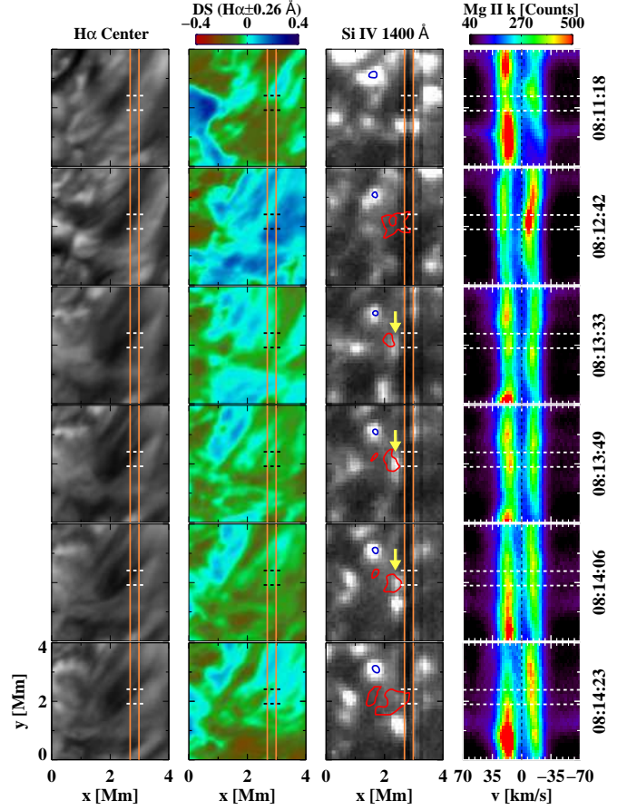
Fig. 6. Simultaneous H\alpha and UV observations of the vortex region. The H\alpha line center images (column 1), DS maps at H\alpha\pm 0.26 \text{ \AA} (column 2), IRIS Si IV 1400 \text{ \AA} SJIs (column 3) of the ROI, as well as the respective IRIS Mg II k 2796 \text{ \AA} spectra (column 4), are shown at certain times before and during the two upflow events. The red and blue contours on the SJIs represent the two spiral arms of the vortex and their neighboring bright point seen in the H\alpha-0.77 \text{ \AA} images, respectively. The IRIS slit is indicated with two vertical lines in each panel in columns 1–3. A subregion on the slit is shown with a dashed strip in each panel, which is used for determining the mean line profiles of Mg II k 2796 \text{ \AA} and subordinate Mg II 2798.8 \text{ \AA} lines in Fig. 7. A positive (negative) Doppler velocity corresponds to an upflow (downflow).
