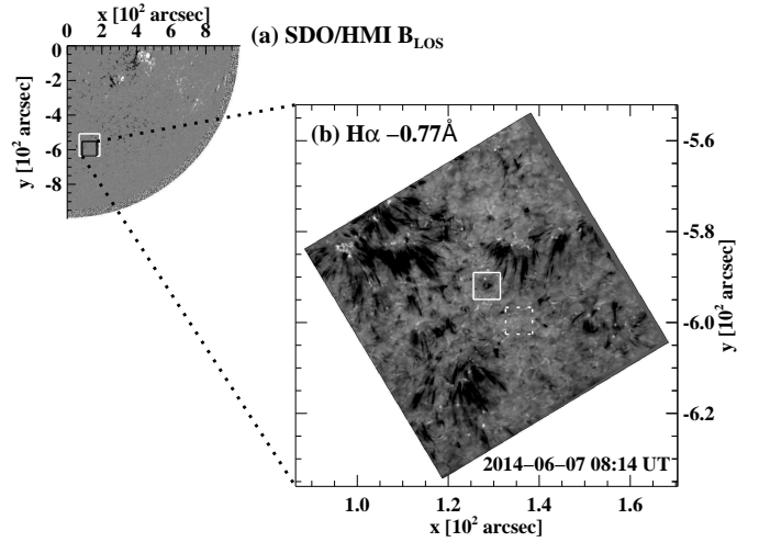
Fig. 1. (a) HMI line-of-sight magnetogram with the FOVs of the CRISP and IRIS observations overlotted in black and white rectangles, respectively. (b) A sample of the cotemporal CRISP FOV H\alpha - 0.77 \text{ \AA} image. The overlotted white solid and dashed rectangles in panel b indicate the ROI (i.e., the FOV of Figs. 2–4a and column 1–3 of Fig. 6) and a neighboring typical quiet Sun region considered in determining the average H\alpha line reference profile, respectively.
