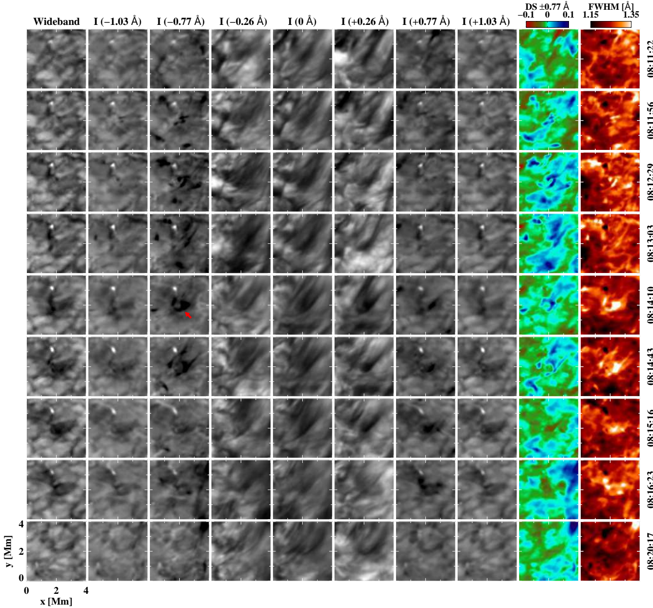
Fig. 2. Sequence of the H\alpha wideband (column 1) and narrowband (columns 2–8: -1.03 \text{ \AA} , -0.77 \text{ \AA} , -0.26 \text{ \AA} , the H\alpha line center, +0.26 \text{ \AA} , +0.77 \text{ \AA} and +1.03 \text{ \AA} ) images of the ROI, which is indicated with a solid box in Fig. 1b, including the respective maps of DS at \pm 0.77 \text{ \AA} (column 9) and FWHM (column 10). Respective times of observation are shown along the right ordinate. This figure is accompanied by an on-line movie. The rightmost column for the FWHM, which is present in Fig. 2, is not included in the movie.
