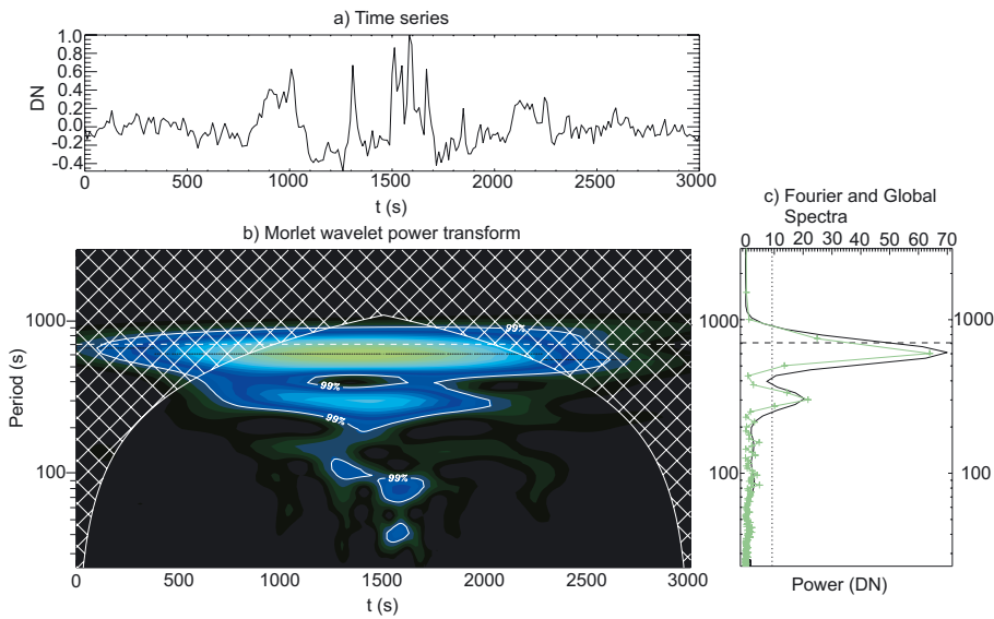
Fig. 9. Similar to Fig. 8 expect the analysed time series is from the 304 Å cross-cut.
