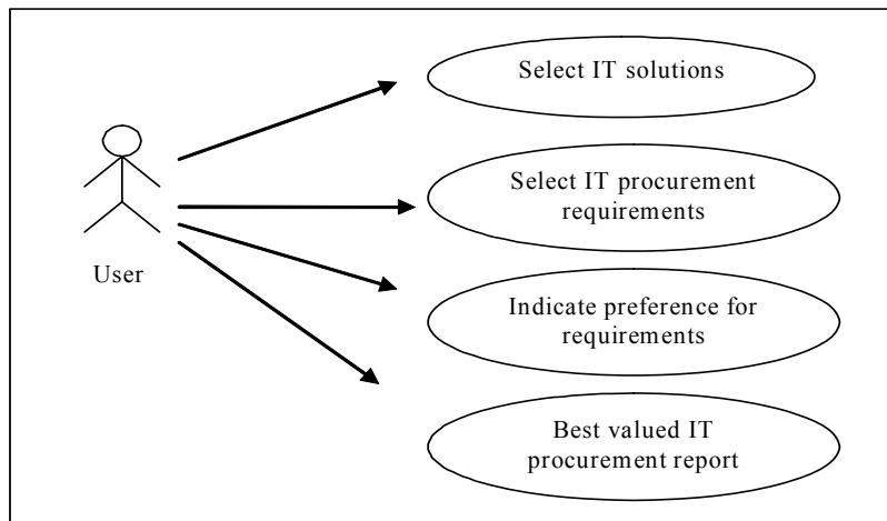
Figure 7: Use-case diagram
