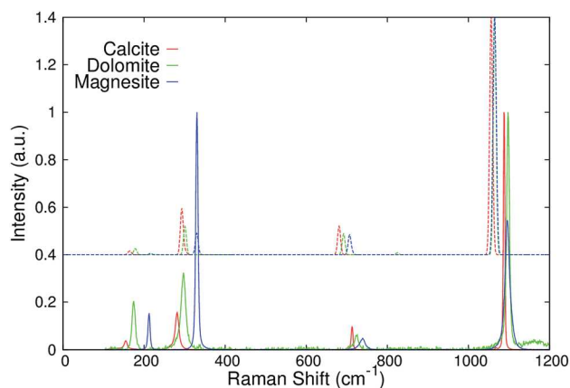
Fig. 2 Comparison of experimental (full lines) and simulated (dashed lines, offset) for carbonate minerals, calcite, dolomite and magnesite. Below 600\text{ cm}^{-1} there is excellent agreement between the simulated and experimental spectra. At higher frequencies a shift is observed but the order of peaks seen for the different minerals is reproduced.
