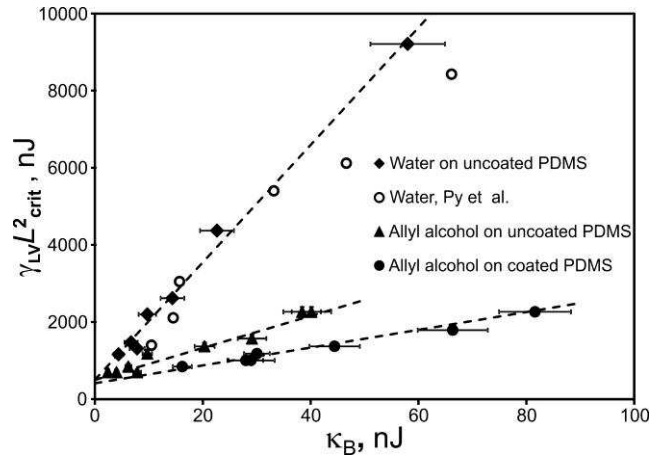
FIG. 4. The variation of \gamma_{\text{LV}}L_{\text{crit}}^2 with \kappa_{\text{B}} for water on uncoated PDMS (filled diamonds), and allyl alcohol on uncoated PDMS (filled triangles) and coated PDMS (filled circles). The open circles show Py et al's. 6 data for comparison.
