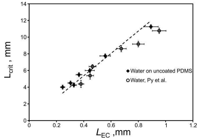
FIG. 3. The dependence of L_{\text{crit}} for wrapping water droplets on uncoated PDMS on L_{\text{EC}} (filled diamonds). The open circles show the corresponding data of Py et al. 6 for comparison.
