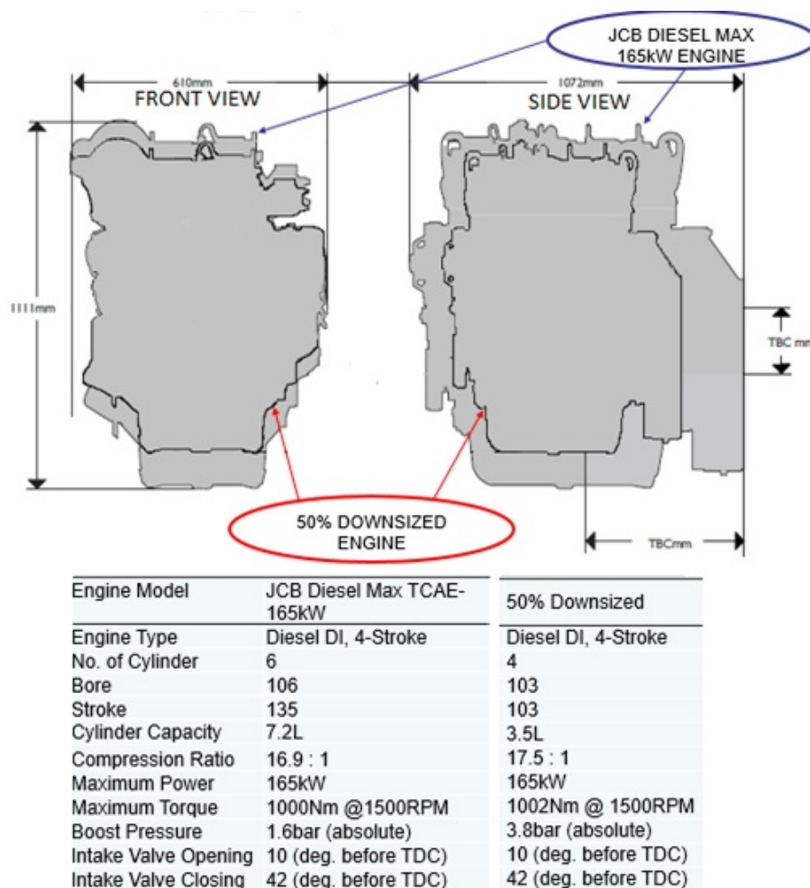
Figure 9. Comparison of engine parameters for reference and 50% downsized engine.
