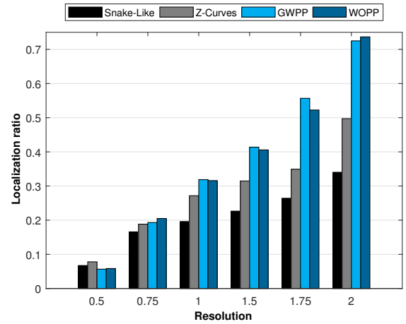
Figure 11: Localization ratio versus the resolution of all mobility models in both WCL and WCWCL
