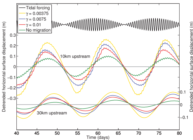
Figure 5. Comparison of detrended in-line displacements for geometries with different slopes. The upper plot shows the tidal forcing (scaled down by a factor of 100 and shifted vertically for clarity). The middle plot shows in line displacements 10 km upstream of the grounding line with and without migration, and the lower plot shows the same 30 km upstream.
