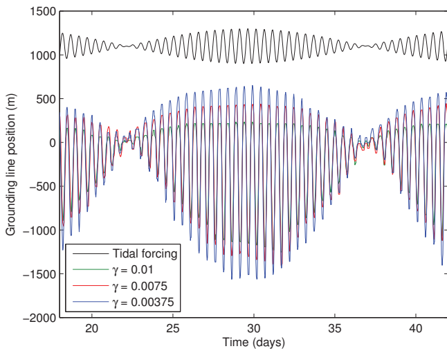
Figure 4. Comparison of change in grounding line position from the mean location, for various slopes ( \gamma ) as a function of time. The tidal forcing is also shown (solid black line), scaled up and shifted vertically.
