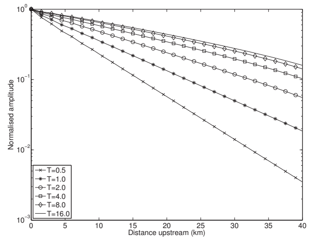
Figure 7. Normalised amplitude response to various periods (in days) of boundary forcing as a function of distance upstream as calculated by the model. Model parameters used were A = 4.0 \cdot 10^{-7} \text{ d}^{-1} \text{ kPa}^{-1} , m = 1 , n = 1 , E = 3 \text{ GPa} , \nu = 0.45 and a value for the rate factor in the till to produce surface velocities of 1 \text{ m d}^{-1} . Note that amplitude is plotted on a log scale.
