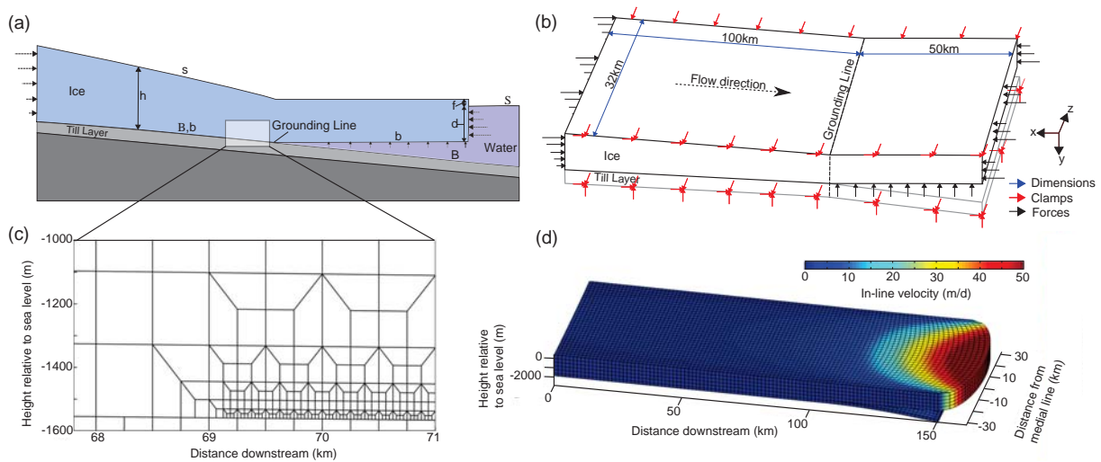
Figure 1. Model setup for 2-D (a, c) and 3-D (b, d) simulations. Panels (a) and (b) are schematic representations of the model domains while (c) and (d) show the model grid (panel (c) is zoomed in to show refinement near the grounding line). The 3-D grid in (d) has been vertically exaggerated by a factor of 4.
