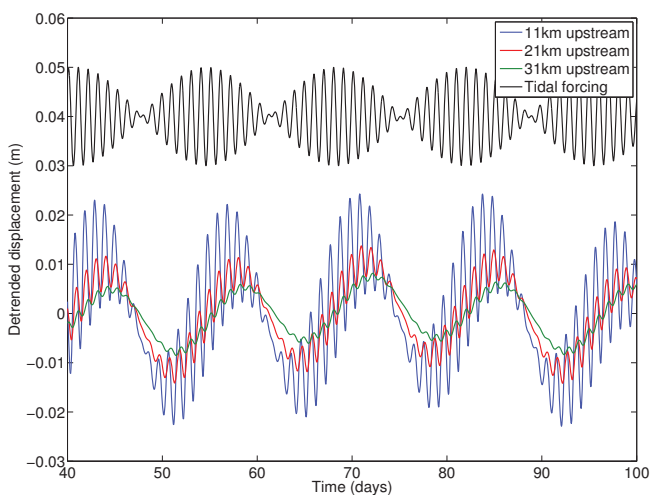
Figure 3. Detrended in-line displacements at 11, 21 and 31 km upstream of the grounding line for the 3-D model run using an idealised Siple coast geometry. The tidal forcing is also shown, scaled down by a factor of 100 and shifted vertically.
