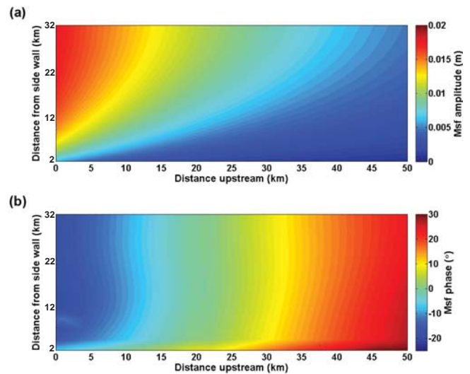
Figure 6. Plots showing amplitude (a) and phase (b) of the Msf tidal constituent based on tidal analysis of detrended horizontal surface displacement.
