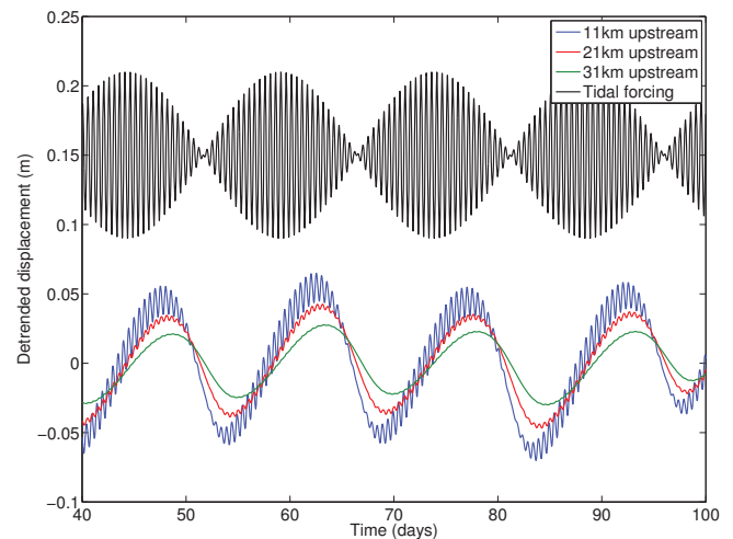
Figure 2. Detrended in-line displacements at 11, 21 and 31 km upstream of the grounding line for the 3-D model run using an idealised ice stream geometry. The tidal forcing is also shown, scaled down by a factor of 100 and shifted vertically.
