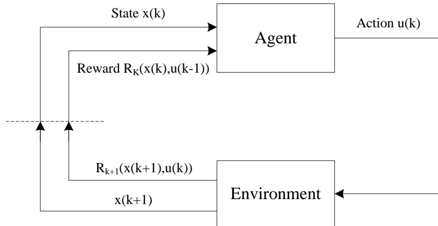
Figure 2. The basic frame of reinforcement learning.
