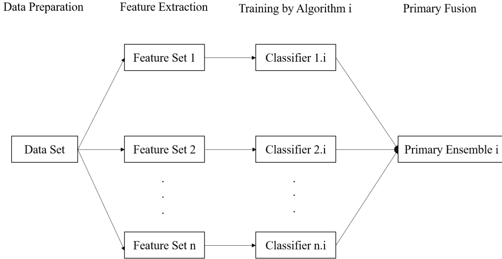
Figure 3: Procedure of Primary Ensembles Creation
