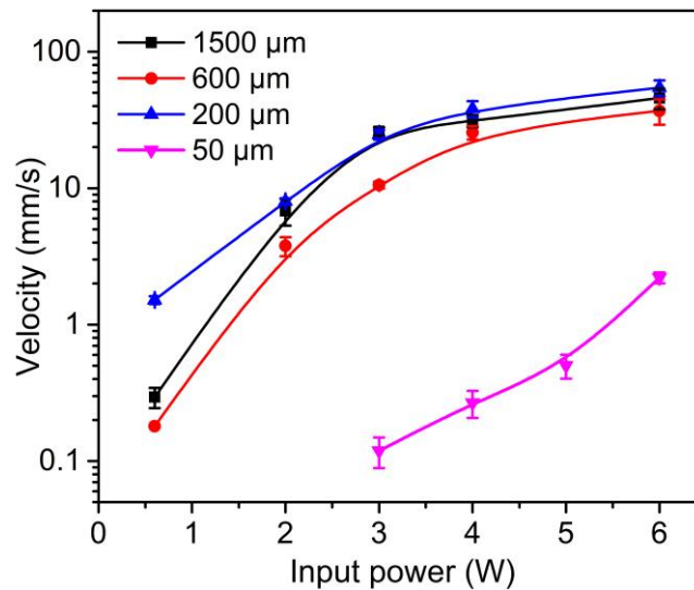
Figure 5. Droplet (1 \mu\text{L} ) average pumping velocities as a function of input power, for thick Al plate (i.e., 600 \mu\text{m} and 1500 \mu\text{m} ) SAW devices driven using the Rayleigh mode, for thin Al sheet (200 \mu\text{m} thick) and Al foil (50 \mu\text{m} thick) SAW devices driven using pseudo- R_0 or A_0 mode.
