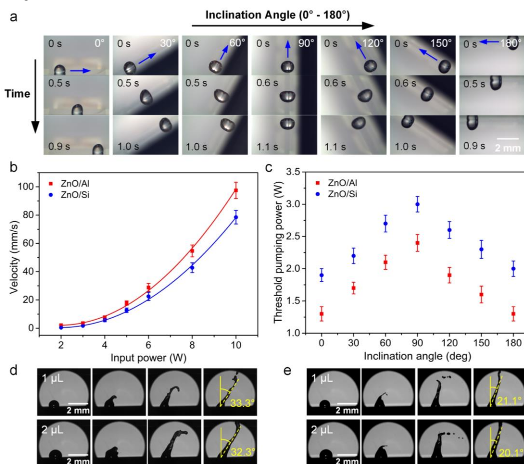
Figure 4. (a) Droplet (1 \mu\text{L} ) pumping images along inclined surfaces with inclination angles from 0^\circ to 180^\circ using ZnO/Al plate SAW device with an input power of 5 W. (b) Comparisons of average pumping velocities for the droplet on the flat surface under different input powers between ZnO/Al plate SAW device and ZnO/Si SAW device. (c) Threshold powers of pumping a 1 \mu\text{L} droplet for ZnO/Al plate SAW device and ZnO/Si SAW device under different inclination angles. High-speed images indicating the jetting angles using (d) ZnO/Al plate SAW device and (e) ZnO/Si SAW device with the same input power of 18 W.
