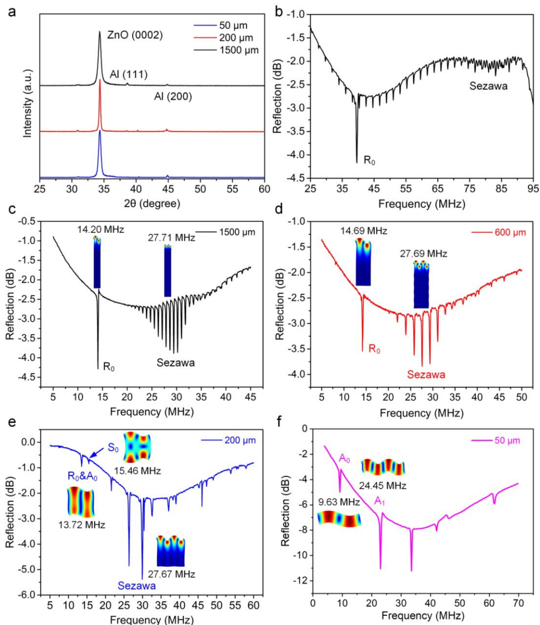
Figure 2. (a) XRD patterns of ZnO thin films on various thick Al sheet substrates. (b) Signal reflection spectra ( S_{11} ) of ZnO/Al plate (1500 \mu\text{m} thick) SAW device with the wavelength of 64 \mu\text{m} . FEA simulation and experimental verification of wave vibration modes and their corresponding resonant frequencies for the SAW devices with 200 \mu\text{m} wavelength and varied Al sheet thicknesses of (c) 1500 \mu\text{m} , (d) 600 \mu\text{m} , (e) 200 \mu\text{m} and (f) 50 \mu\text{m} .
